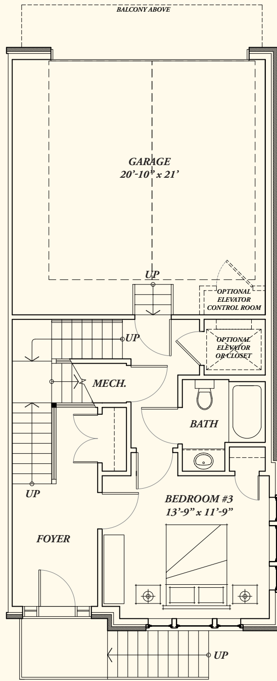
ALT. GROUND FLOOR
