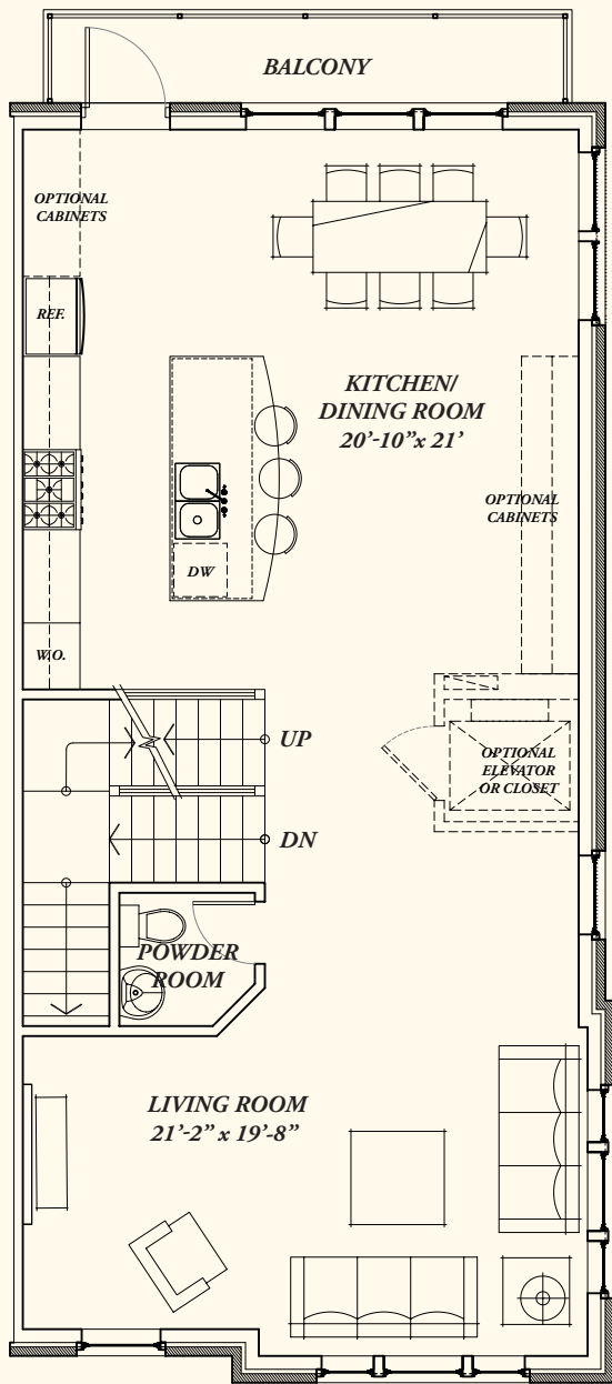
ALT. SECOND FLOOR
